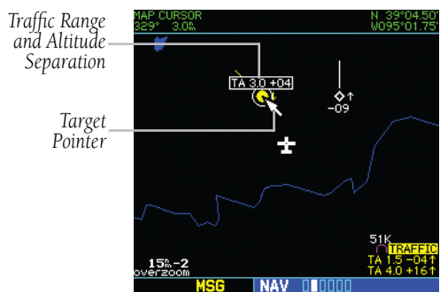
Figure 14-18 Traffic Range and Altitude Separation
