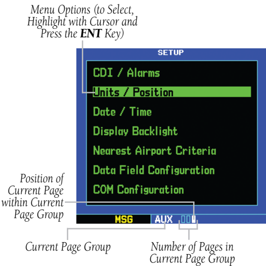
Figure 10-28 Setup Page
