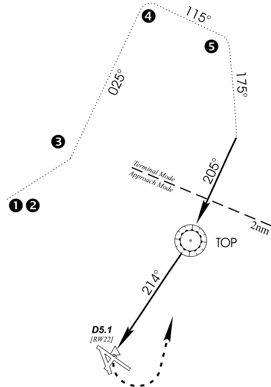
Figure 6-43 Terminal Mode
