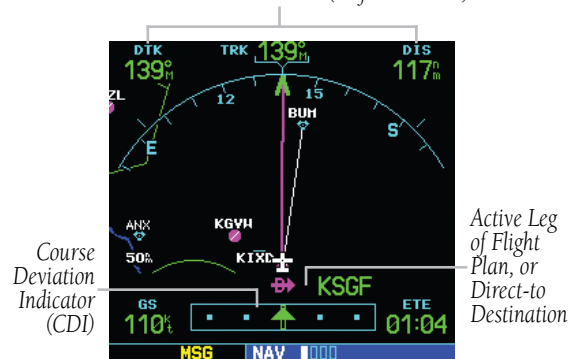
Figure 1-18 Default NAV Page
